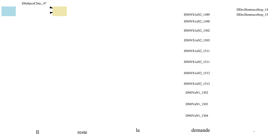
Fig. 1. Initial automaton provided by an IG for the sentence " Il reste la demande. ". There are initially 7392 way of tagging the sentence.
