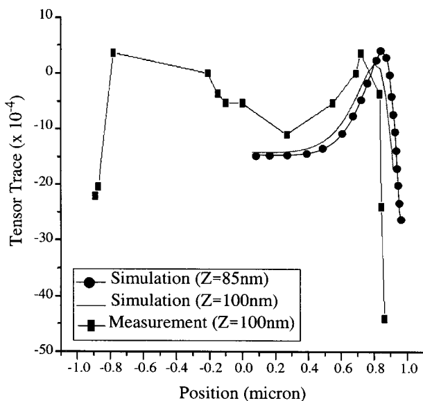
FIG. 11. Comparison between the calculated and measured trace of the strain tensor as a function of the lateral position in the 2- \mu\text{m} -wide STI structure along a cut line at z=100\text{ nm} below the silicon/silicon dioxide interface. The numerical calculations are performed with an elastic model of the rheological behavior of silicon.
