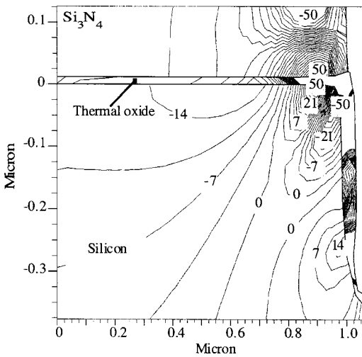
FIG. 10. 2D calculated distribution of the trace of the strain tensor in the 2- \mu\text{m} -device of the structure shown in Fig. 6. Strain values are divided by 1 \times 10^{-4} .
