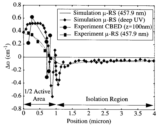
FIG. 12. Comparison between the Raman shifts obtained from: (1) simulated \mu\text{RS} experiment (457.9 nm, no symbol), (2) simulated \mu\text{RS} experiment (deep UV, diamond), (3) CBED experiment (cut line at z=100\text{ nm} under the Si/SiO 2 interface, circle), and (4) real \mu\text{RS} experiment (457.9 nm, square) in the 2- \mu\text{m} -wide STI structure.
