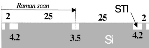
FIG. 6. Schematic picture of the sample used for Raman spectroscopy experiments. It consists of 2- and 25- \mu\text{m} -wide Si lines isolated by shallow trenches (STI). The arrow indicates the region scanned by Raman spectroscopy. It crosses first a 2- \mu\text{m} -wide Si line and next a 25- \mu\text{m} -Si line. The results of this measurement are shown in Fig. 7.
