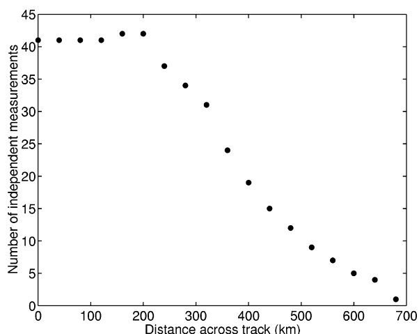
FIG. 2. Number of independent ( T_v , T_h ) measurements in pixels resampled at 40 km across track, from the center to the edge of the swath; note that the number of independent measurements is twice the one plotted in the figure (dual polarization).
