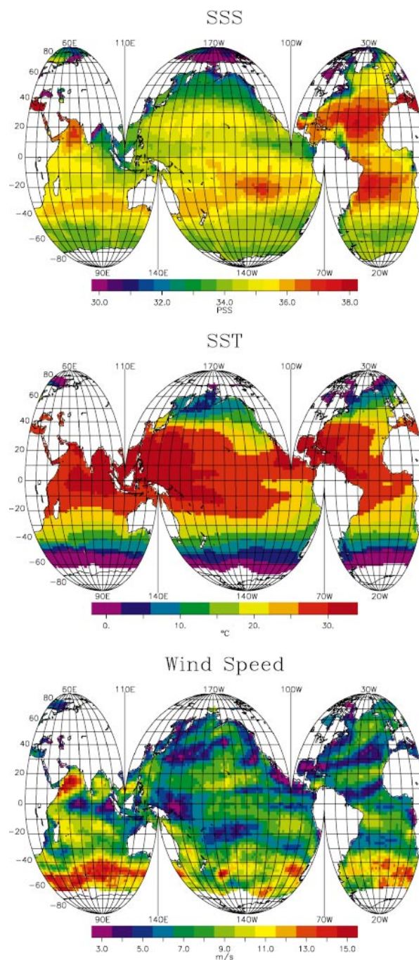
FIG. 7. Global maps of (top) SSS for Jul, (middle) SST from 15 to 29 Jul 1999, and (bottom) 10-day average wind speed from 21 to 31 Jul 1999, illustrating the environmental conditions at the time of the error simulation.
