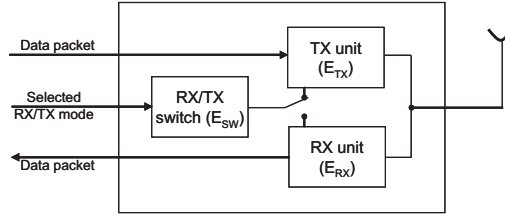
Figure 5: Energy radio transceiver model.
