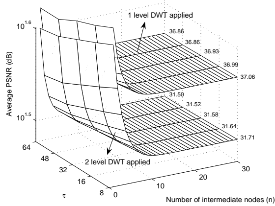
Figure 10: Average PSNR for semi-reliable transmission and coefficients magnitude based discarding strategy.
