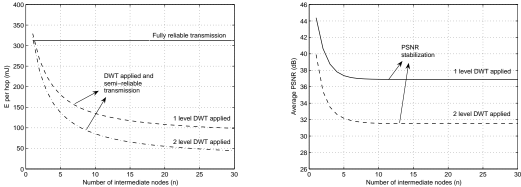
(a) Average energy consumption for semi-reliable transmission and resolution-based priorities. (b) Average PSNR for semi-reliable transmission and resolution-based priorities.
