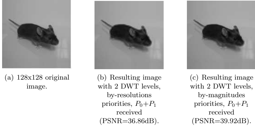
Figure 12: Comparison of resulting images by applying different prioritization strategies and packet discarding.
