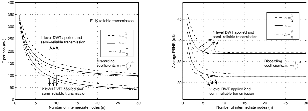
(a) Average energy consumption for 1 and 2 level DWT. (b) Average PSNR for 1 and 2 level DWT applied.
