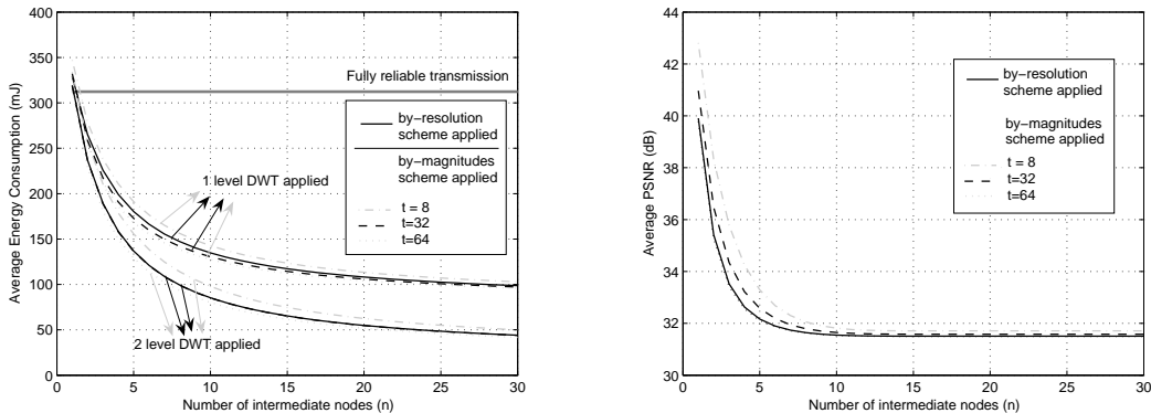
(a) Comparison of average energy consumption for resolution-based and magnitudes-based priorities and semi-reliable transmission. (b) Comparison of average PSNR for resolution-based and magnitudes-based priorities and semi-reliable transmission.
