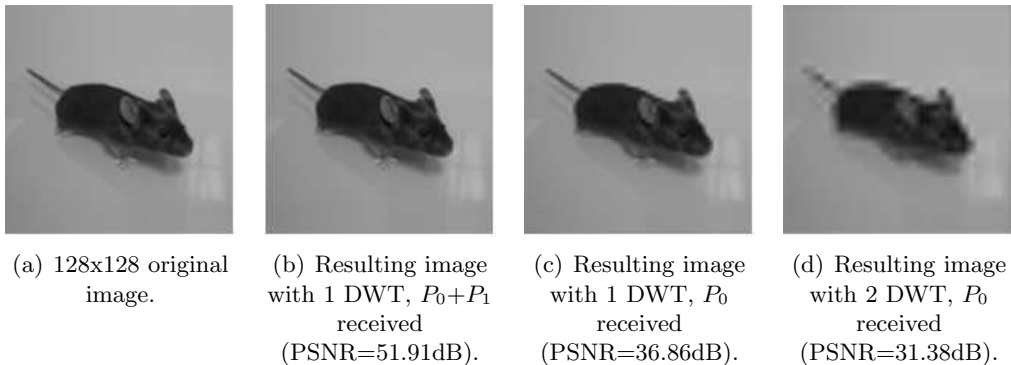
Figure 8: Resulting images with DWT applied.
