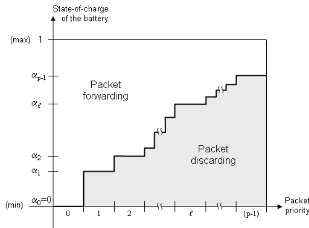
Figure 2: Packet forwarding policy based on priorities.
