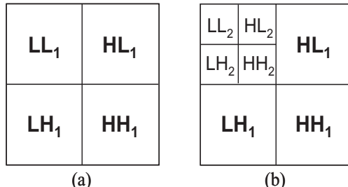
Figure 1: 2-D DWT applied once (a) and twice (b).
