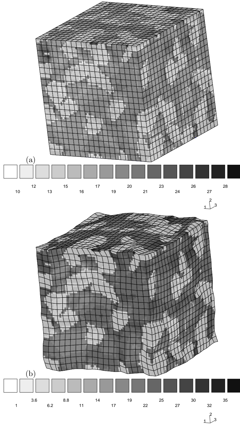
Figure 5: Contour of von Mises equivalent stress (in MPa): (a) Transient regime (at t = 400s ), (b) steady state (at t = 30000s ). The macroscopic shear stress \Sigma_{12} = 10MPa was applied.
