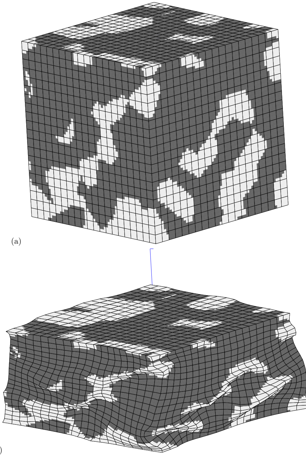
Figure 10: Morphology changes during compression creep (overall compression strain: 15%), White color: Mw, Grey color: Mg-Pv, (a) initial state, (b) deformed state.
