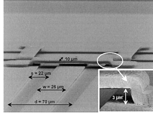
Fig. 1. Bridges on a 50- \Omega CPW, T-junction discontinuity.
