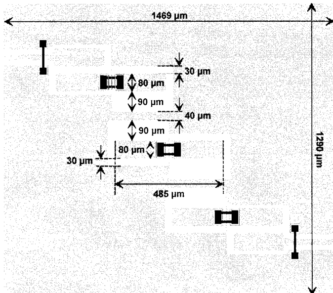
Fig. 10. Layout of a 94-GHz central-frequency, 5% 3-dB-bandwidth, coupled-line filter.
