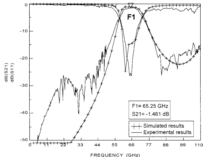
Fig. 9. Simulated and experimental magnitude responses of the 65-GHz central-frequency, 22% 3-dB-bandwidth, coupled-line filter.
