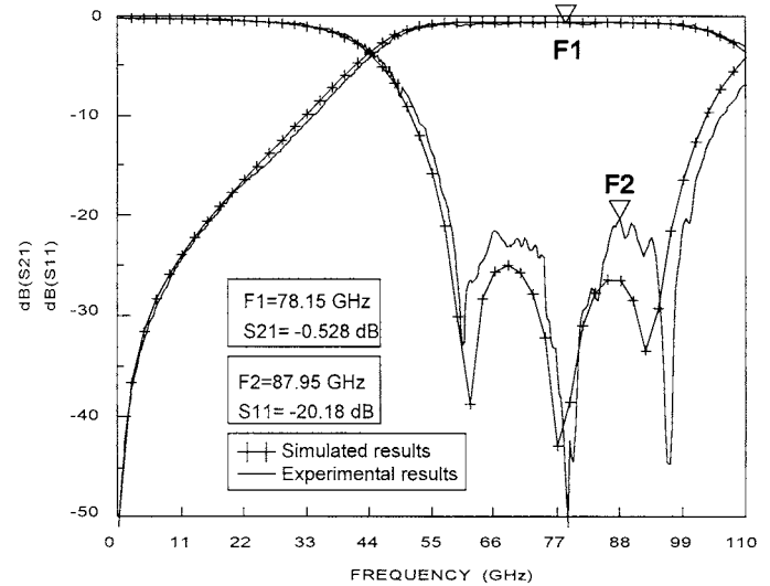
Fig. 5. Simulated and experimental magnitude responses of the 78-GHz central-frequency, 82% 3-dB-bandwidth filter.
