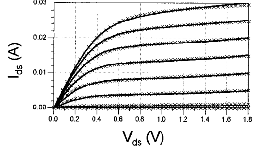
Fig. 2. Static drain current versus V_{ds} for different values of V_{gs} (0–1.8 V/0.2 V). Symbols correspond to the measurements and the solid line to the simulation.
