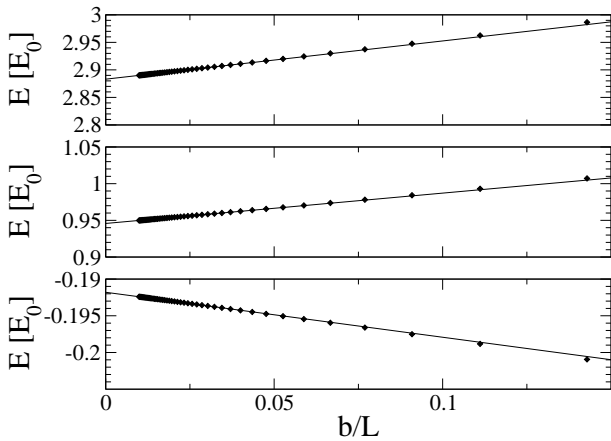
FIG. 1: First three eigenenergies for the interacting states of two fermions in a box of size L for an infinite scattering length in the lattice model, as functions of the lattice period b . The total momentum of the eigenstates is fixed to zero. The computed eigenenergies are given by the plotting symbols, in units of E_0 = (2\pi\hbar)^2/2mL^2 ; the straight lines are linear fits performed on the data with b/L < 2 \times 10^{-2} .
