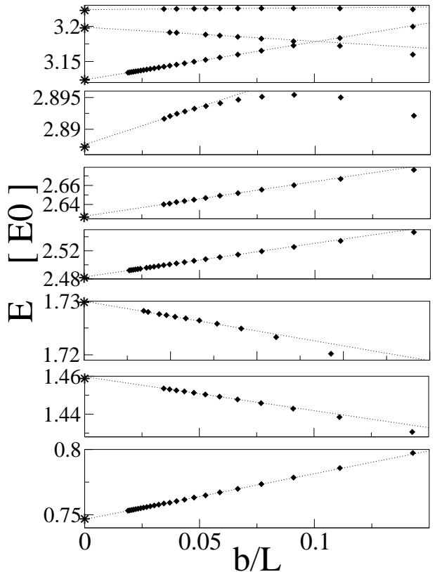
FIG. 2: First eigenenergies of three fermions in a box of size L for an infinite scattering length in the lattice model, for a zero total momentum. The computed eigenenergies (diamonds) are given in units of E_0 = (2\pi\hbar)^2/2mL^2 for different values of the lattice period b . For functions f(\mathbf{r}) invariant by reflection along x, y, z and by arbitrary permutation of x, y, z we have computed the eigenenergies down to smaller values of b/L . The straight lines are a linear fit performed on the data over the range b/L \leq 1/15 , except for the energy branch E \simeq 2.89E_0 which becomes more slowly linear than the other branches. The eigenenergies predicted by the Bethe-Peierls model are given by stars in b = 0 .
