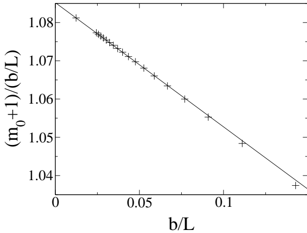
FIG. 3: Quantity (m_0 + 1)/(b/L) as a function of the lattice period b . Here m_0 is the lowest eigenvalue of the matrix M(E) defining the linear system Eq.(21), for E = 0 and for an infinite scattering length. The fact that m_0 + 1 > 0 shows that there is no negative eigenenergy for the three fermions, see text. The symbols are obtained from a numerical calculation of m_0 . The solid line is a linear fit over the range b/L \leq 1/29 , not including the point with b/L = 1/81 : for this point, the matrix M has more than half a million lines so that m_0 was obtained by a computer memory-saving iterative method rather than by a direct diagonalisation.
