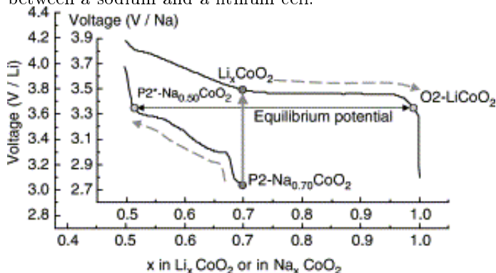
Figure 9: The VOLTAGE= f(x) electrochemical curves obtained for the Li//Li x CoO 2 and Na//Na x CoO 2 systems. Note that for a given phase, an 0.3 V difference in potential is observed between a sodium and a lithium cell.
