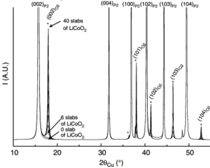
Figure 7: XRD patterns calculated for P2-O2 intergrowths. * indicates the O2-LiCoO 2 peak positions. The average size of the O2 domains varies from 0 to 40 slabs.
