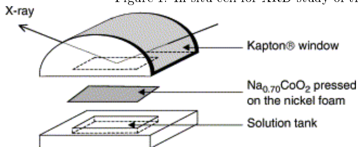
Figure 1: In situ cell for XRD study of the exchange reaction
