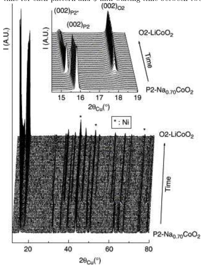
Figure 2: XRD patterns recorded in situ during the exchange of sodium by lithium in P2- \text{Na}_{0.70}\text{CoO}_2 . A total of 64 XRD patterns was recorded during 16 h, with 10 min acquisition time for each pattern and 5 min waiting time between two patterns.
