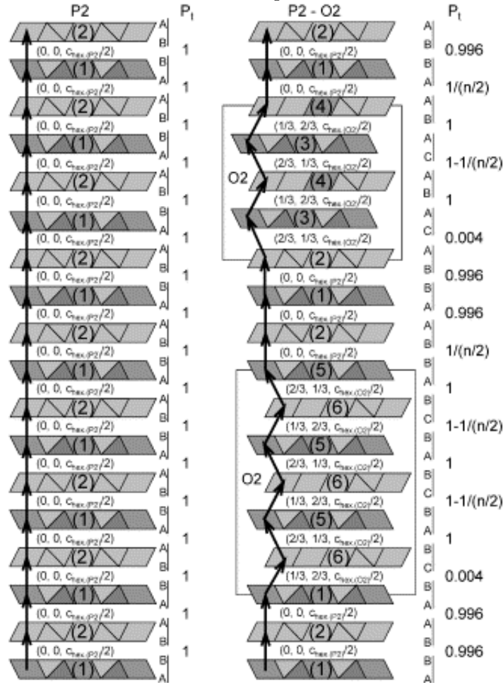
Figure 6: Scheme of the structural models used by DIFFaX software in order to simulate the XRD pattern for pure P2 phase (a) and for P2-O2 intergrowth (b). The stacking vectors and the associated probabilities are also given.
