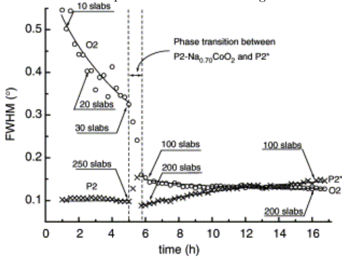
Figure 4: Evolution of the FWHM of the (002) diffraction lines for the P2-Na 0.70 CoO 2 , P2*-Na 0.50 CoO 2 and O2-LiCoO 2 phases, during the ion-exchange reaction. The coherence lengths, calculated from experimental FWHMs using the Scherrer formula, are also given.
