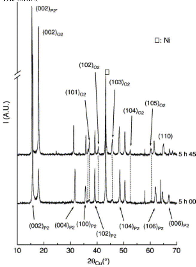
Figure 3: Comparison of the XRD patterns recorded just before and just after the P2→P2* phase transition.
