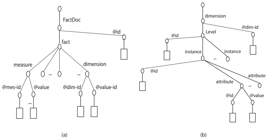
FIG. 3 – facts.xml (a) and dimension_d.xml (b) structure
