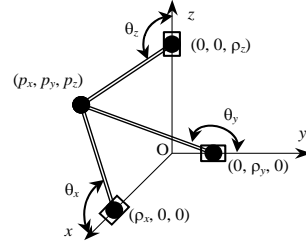
Fig. 2. Orthoglide geometrical model
