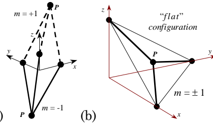
Fig. 7. Double (a) and single (b) solutions of the direct kinematics
