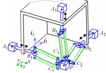
Fig. 1. Orthoglide architecture
