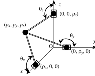
Fig. 2. Orthoglide geometrical model
