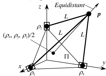
Fig. 6. Geometrical solution of the direct kinematics
