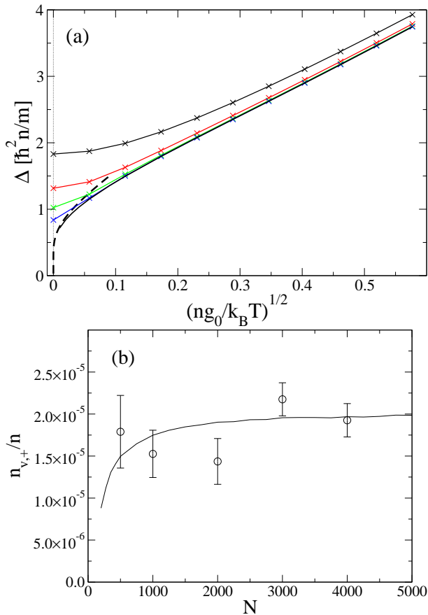
FIG. 11: (Color online) (a) Activation energy \Delta(T) as a function of (g_0 n/k_B T)^{1/2} at a fixed particle density n for increasing system size L/\lambda_{\text{th}} = 6, 12, 24, 48 (thin solid lines, respectively black, red, green, blue, from top to bottom; the crosses are the actually calculated values and the lines are a guide to the eye). The dashed line is the upper bound Eq.(78) for an infinite system size. The thick solid line is the improved upper bound discussed around Eq.(79), plotted for (ng_0/k_B T)^{1/2} \geq 0.01 . (b) Vortex density as a function of the total particle number (for increasing system sizes) for fixed values of the density n and the temperature T = 0.5 T_d/(2\pi) \simeq 0.08 T_d , and a coupling constant g_0 = 0.333 \hbar^2/m . Circles: semi-classical simulations. Solid line: prediction of the activation law 0.44 e^{-\Delta/k_B T} where the numerical factor 0.44 was fitted to the data.
