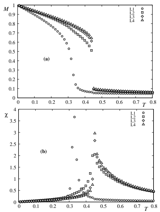
FIG. 5: Magnetizations and susceptibilities of first two cells vs temperature for J_s = -0.5 with L = 24 and D = 0.1 . L_j denotes the sublattice magnetization of layer j . The susceptibility of sublattice 1 of the first cell is divided by a factor 5 for presentation convenience.
