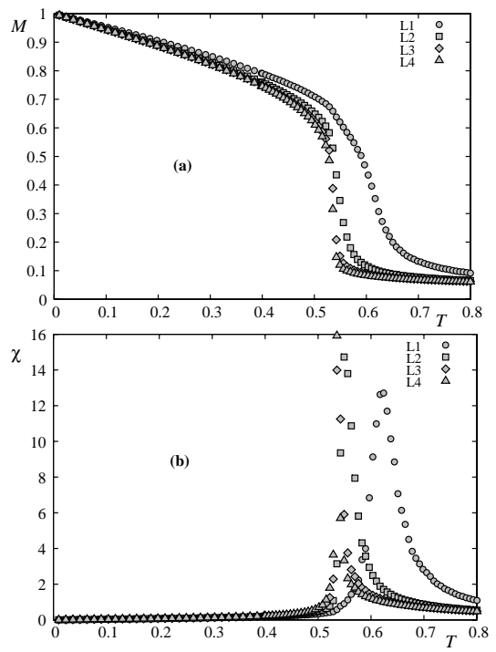
FIG. 3: Magnetizations and susceptibilities of sublattices 1 and 3 first two cells vs temperature for J_s = -1.0 with L = 24 and D = 0.1 . L_j denotes the sublattice magnetization of layer j .
