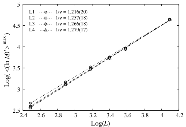
FIG. 12: The maximum value of \langle (\ln M)' \rangle = \langle E \rangle - \langle ME \rangle / \langle M \rangle versus L in the \ln - \ln scale for J_s = -0.1 , where M is the sublattice order parameter. The slope of each line gives 1/\nu . L_j denotes the sublattice magnetization of layer j .
