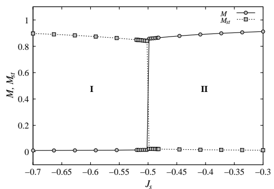
FIG. 8: The magnetization M and the staggered magnetization M_{st} of first layer versus J_s are shown, at T = 0.15 , with L = 24 and D = 0.1 . I and II denote ordering of type I and II defined in Fig. 2. III is paramagnetic phase. See text for comments.
