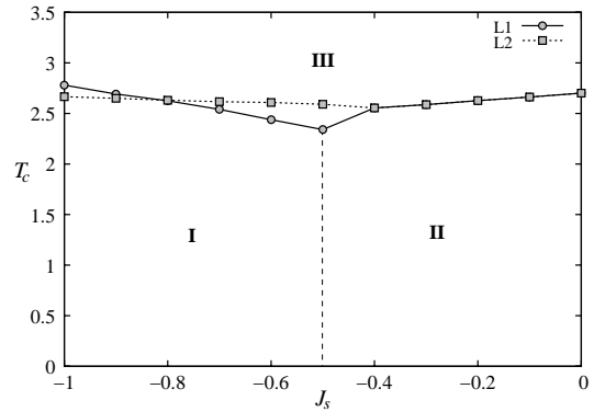
FIG. 19: Phase diagram obtained by the Green's function method with D = 4 . L_j denotes the transition temperature of the sublattice magnetization of layer j . See text for comments.
