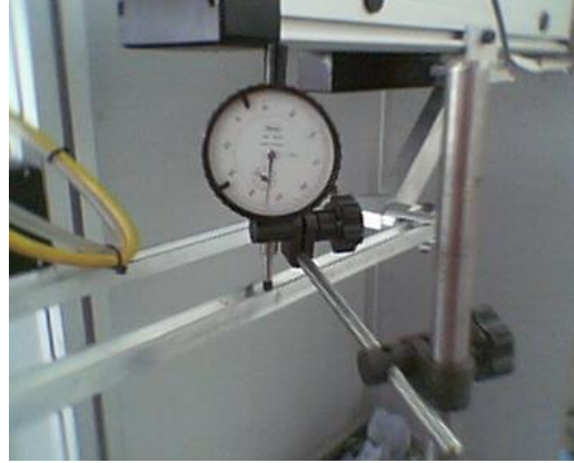
Figure 5: Experimental Setup.
