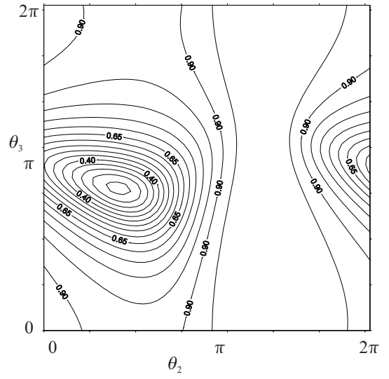
Fig. 13. The isocontours of the objective function of the equilateral manipulator
