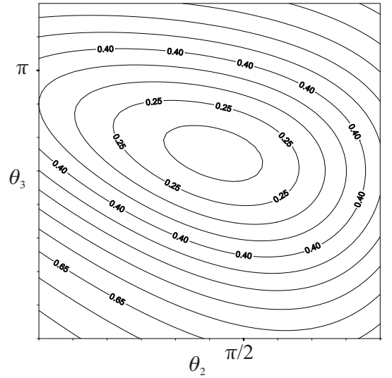
Fig. 15. The isocontours closest to isotropy of the objective function of the equilateral manipulator
