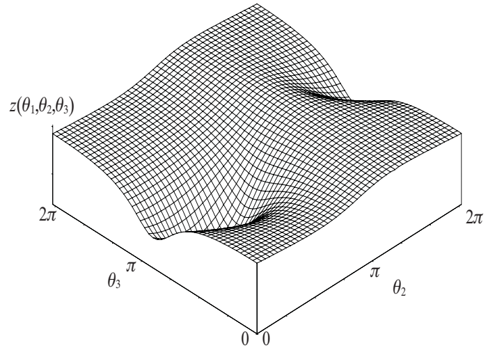
Fig. 11. Objective function of the equilateral manipulator
