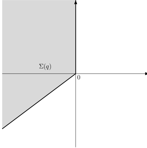
Figure 2: Numerical range \Sigma(q) .
