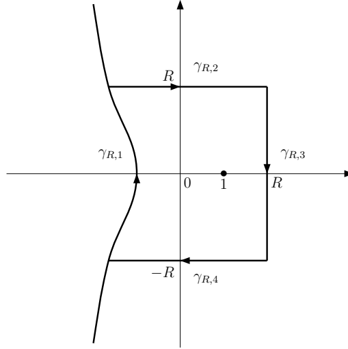
Figure 4: Contour \gamma_R .
