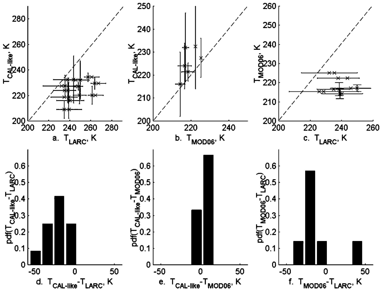
FIG. 3. SIRTAs cloud cases: (a) T_{CAL-like} = f(T_{LARC}) , (b) T_{CAL-like} = f(T_{MOD06}) , (c) T_{MOD06} = f(T_{LARC}) , (d) PDF of T_{CAL-like} - T_{LARC} , (e) PDF of T_{CAL-like} - T_{MOD06} , and (f) PDF of T_{MOD06} - T_{LARC} . Dashed lines are x = y .
