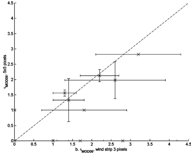
FIG. 2. The \tau_{MOD06} retrieved in the 5 \times 5 pixel area against \tau_{MOD06} retrieved in the 3-pixel-large wind strip, for SIRTAs cases. Error bars are standard deviations calculated in the sample of pixels.
