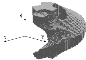
Figure 3 : Octree model of the workspace
