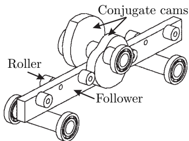
Figure 1: Layout of Slide-o-Cam
