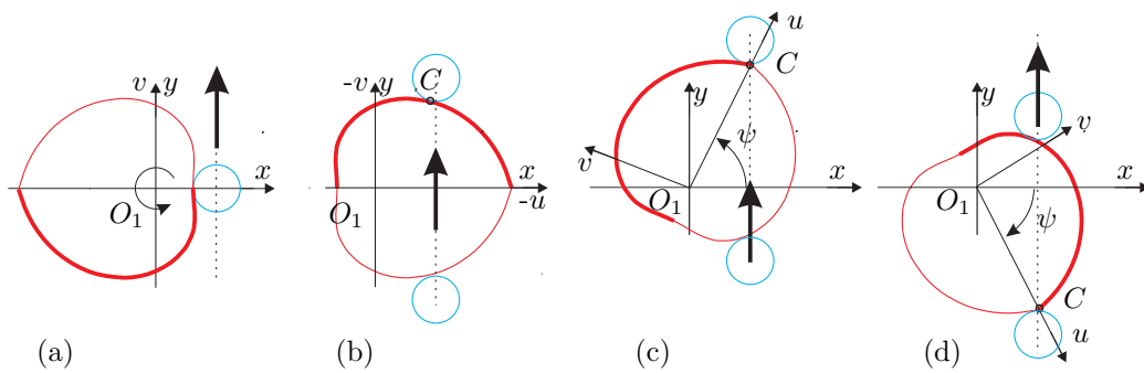
Figure 5: Extended angle \Delta for different values of \psi , for a cam with one lobe: (a) \psi = \pi ; (b) \psi = 2\pi ; (c) \psi = 2\pi - \Delta ; and (d) \psi = \Delta
