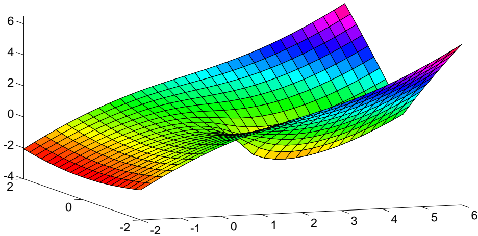
Figure 2: Perspective view of R_0 .
