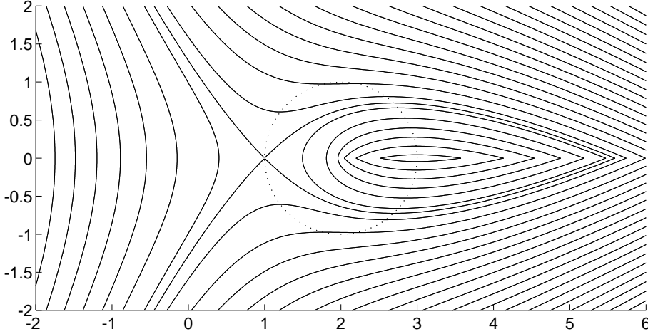
Figure 3: Level curves of R_0 .
