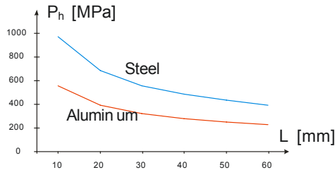
Figure 11: Variation of P_{h_{max}} as a function of L for \phi_{bear} = 6.7mm and \phi_{cam} = 3.8mm for steel and aluminum parts and the Orthoglide constraints
