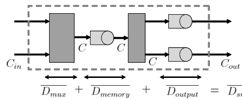
Fig. 1. Model of a 2 port-switch in a full duplex mode based on shared memory and a cut-through management.
