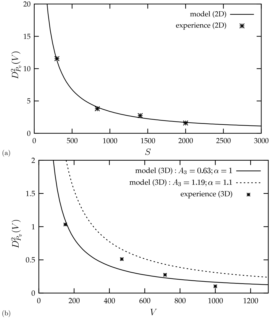
Figure 4: Variance of the apparent property for viscoplasticity P_v as a function of the domain size: simulations and model, (a) 2D ( \alpha = 1; A_2 = 1.3 ), (b) 3D ( \alpha = 1-1.1; A_3 = 0.63-1.19 )
