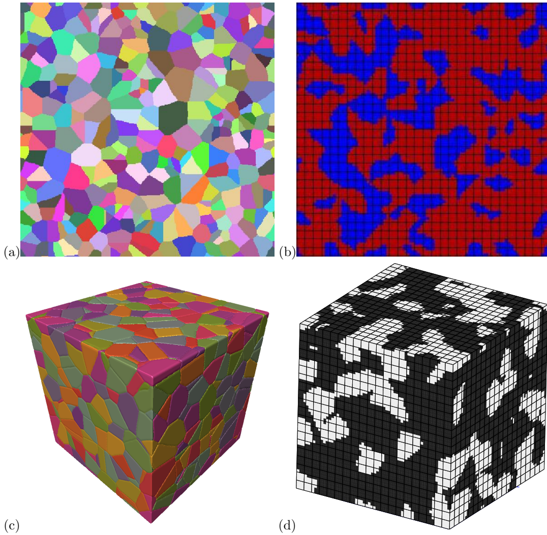
Figure 1: (a) 2D microstructure (Voronoi mosaic containing 300 grains), (b) Meshing of a Two-phase material: 2D Voronoi mosaics containing 300 grains with 70% of phase1 and 30% of phase2, (c) 3D microstructure (Voronoi mosaic containing 470 grains), (d) Meshing of a Two-phase material: 3D Voronoi mosaics containing 470 grains with 70% of phase1 and 30% of phase2.
