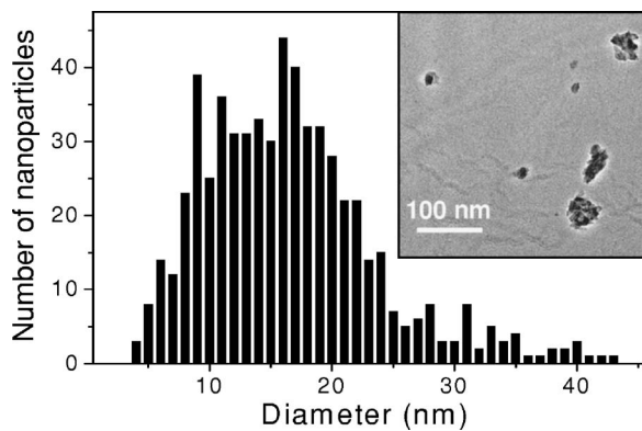
FIG. 1. Size distribution of Y_{0.6}Eu_{0.4}VO_4 nanoparticles determined from TEM images (see inset). Total number of NPs: 603.
