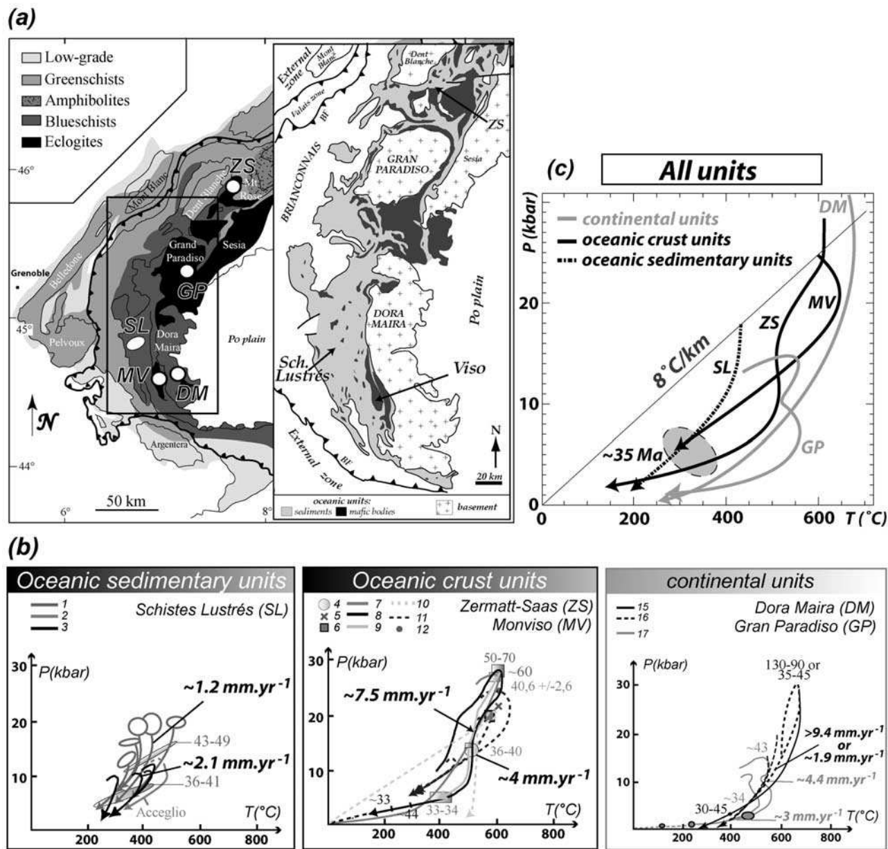
Figure 1. (a) Simplified metamorphic map [after Frey et al., 1999] and location of the units where pressure-temperature-time (P-T-t) paths are taken from. (inset) Map presenting the repartition of the oceanic-derived units. (b) P-T-t paths for oceanic units (black boxes) for (SL) “Schistes Lustrés” unit, (ZS) Zermatt-Saas unit, and (MV) Monviso unit. P-T-t paths of continental units are given for comparison in gray box for (DM) Dora Maira and (GP) Gran Paradiso. Numbers refer to (1) [Agard et al., 2001]; (2) [Schwartz et al., 2000b]; (3) [Schwartz et al., 2000a]; (4) [Ernst and Dal Piaz, 1978]; (5) [Meyer, 1983]; (6) [Barnicoat and Fry, 1986]; (7) [Van der Klauw et al., 1997]; (8) [Reinecke, 1998]; (9) [Amato et al., 1999]; (10) [Widmer and Thompson, 2001]; (11) [Schwartz et al., 2000a]; (12) [Cliff et al., 1998; Messiga et al., 1999]; (15) [Henry et al., 1993]; (16) [Duchêne et al., 1997b]; and (17) [Brouwer et al., 2002]; ages are consistent with Hurford and Hunziker [1989]. (c) Simplified P-T paths for the above units. Some of the P-T paths present a slight heating at about 35 Ma (e.g., Zermatt-Saas zone, Gran Paradiso) coeval with the medium-pressure medium-temperature Lepontine metamorphic overprint of the central Alps (5–7 kbar, 650–700°C; [e.g., Todd and Engi, 1997]), which presumably marked the inception of collisional processes [e.g., Goffé et al., 2003].
