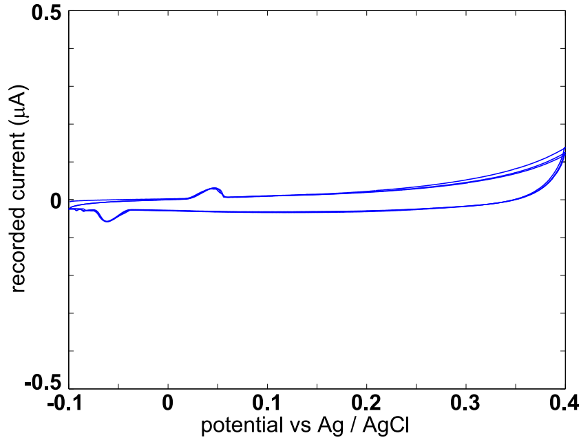
Figure 4. Cyclic voltammetry of the microcantilevers array in a 10^{-2} M KCl solution. Number of cycles: 3, scan rate: 2 mV/s, starting potential: -0.1 V vs. Ag/AgCl.
