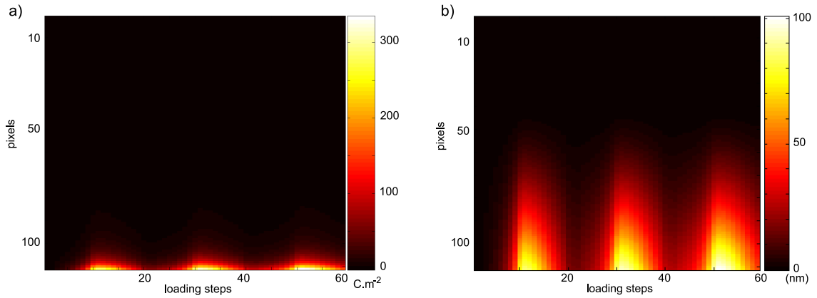
Figure 8. a) Identified charge density field along the median line of the cantilever as a function of the loading step. b) Identified out-of-plane displacement field along the median line of the cantilever as a function of the loading step.
