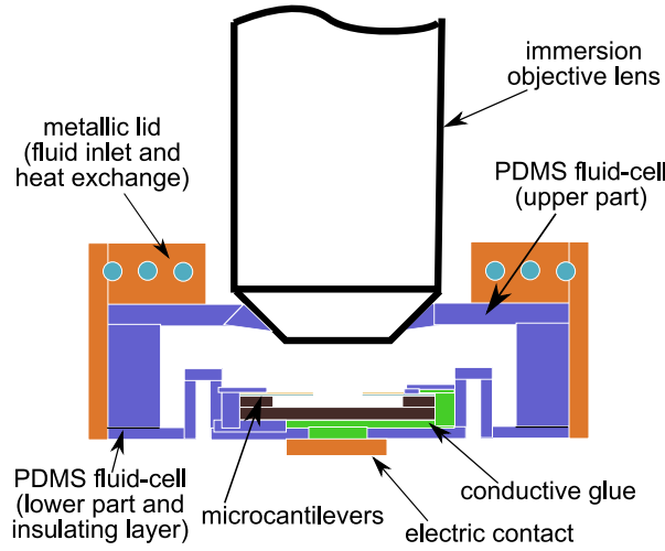
Figure 3. Schematic view of the used fluid cell.
