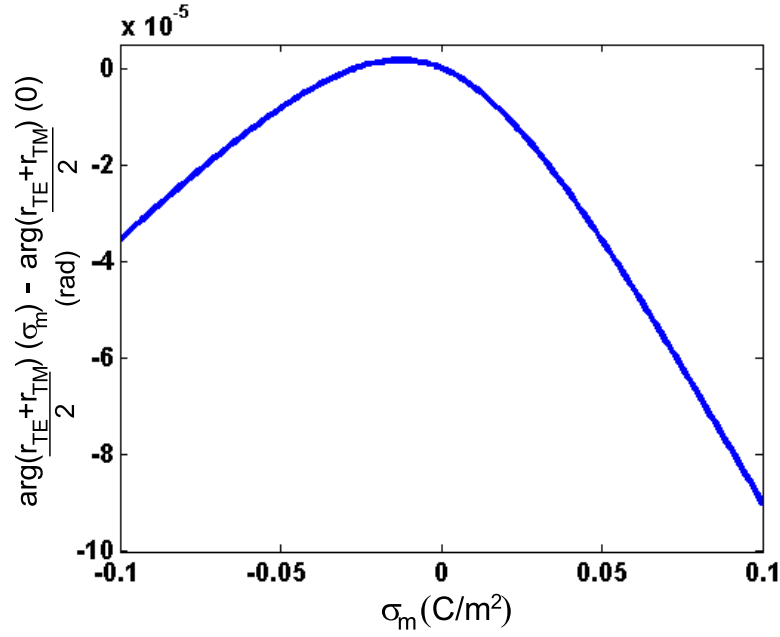
Figure 5. Change of the phase of the base complex reflection coefficient \frac{r_{TE}+r_{TM}}{2} of a Au(111)/KCl interface as a function of the surface charge for \theta_e = 0.3 rad.
