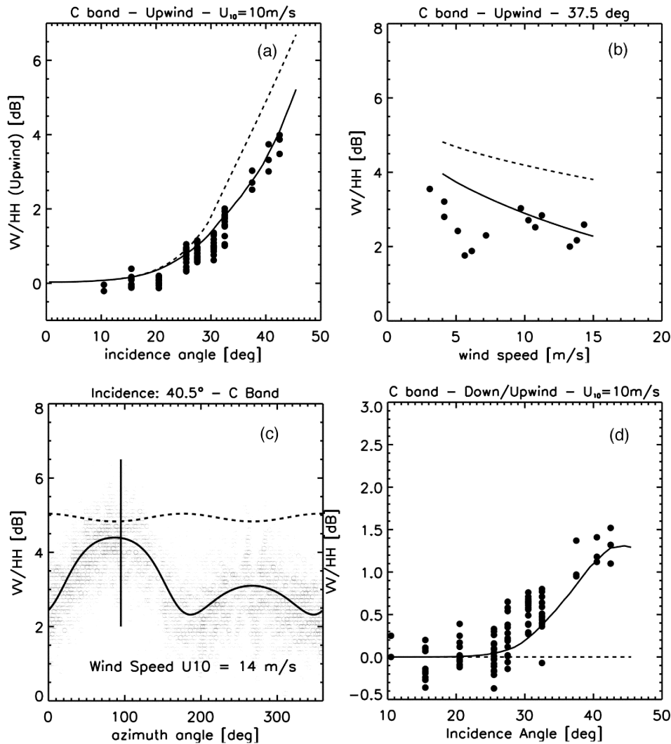
Figure 16. Results for the polarization ratio ( VV/HH ) plotted in dB. (a) As a function of incidence angle for a wind speed of 10 \text{ m s}^{-1} , in the upwind direction. (b) As a function of wind speed for the 37.5^\circ incidence angle. (c) As a function of azimuth angle for the same case as in Figure 3, and the incidence angle of 40.5^\circ . The vertical bar indicates the downwind direction. (d) Downwind to upwind ratio (in dB) of the polarization ratio ( HH/VV ), as a function of incidence angle. In Figures 16a–16d, the dashed line is for the TS + GO model, and the solid line is for the full model including the effect of breaking waves.
