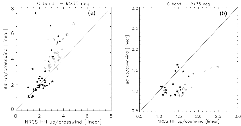
Figure 12. (a) Upwind to crosswind ratio of the NRCS difference (VV-HH) as a function of the upwind to crosswind ratio of the NRCS in HH, for all STORM data points at incidence angles of 37.5° (circles), 40.5° (diamonds), and 42.5° (stars). Solid (respectively open) symbols correspond to wind speed smaller (respectively larger) than 10 m s -1 . (b) Same as Figure 12a, but for the Upwind to downwind ratio of the NRCS difference (VV-HH) as a function of the upwind to downwind ratio of the NRCS in HH. Note that the number of data points in Figure 12a is about twice that in Figure 12b, because observations in two crosswind directions (left and right of upwind) have been used.
