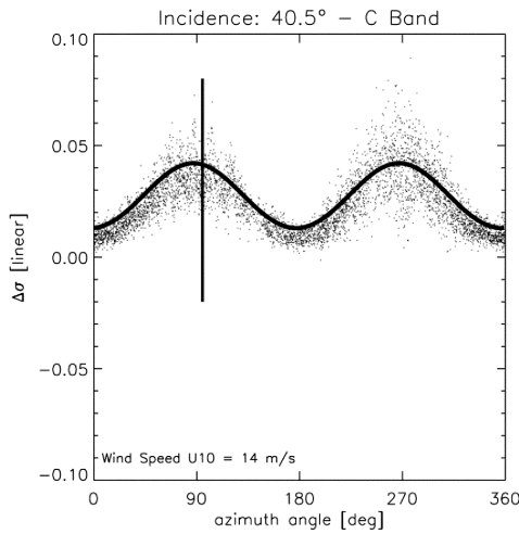
Figure 10. Same as Figure 8, but as a function of azimuth angle for the incidence angle of 40.5^\circ and a case of strong wind ( 14 \text{ m s}^{-1} ). The vertical bar indicates the downwind direction. The TS model using the spectrum of KHCC is plotted as a solid line.
