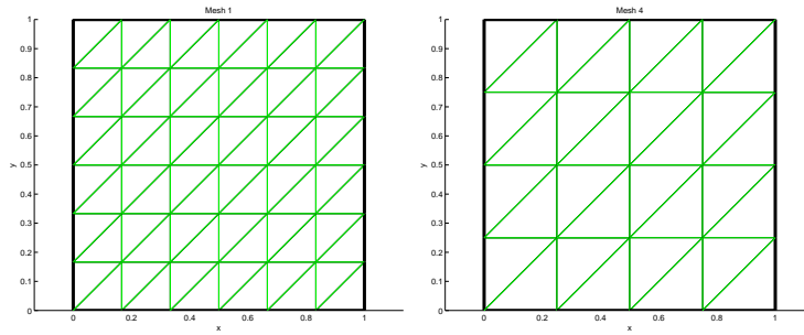
FIG. 4.3. Uniform conforming meshes : mesh 1 (on the left), and mesh 4 (on the right)
