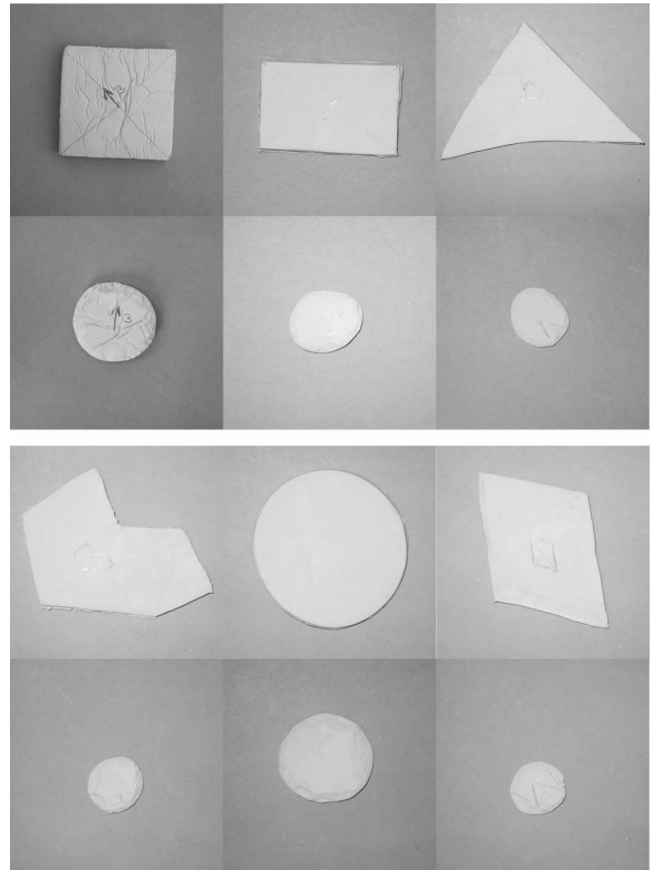
FIG. 5: The initial and final forms of different shapes eroded in our experiment, all shown with the same magnification. The erosion times for the final shapes are 40 min for square, 30 min for rectangle, 30 min for triangle, 35 min for polygon, 35 min for circle, and 30 min for lozenge. Note that the final shapes are all roughly circular.
