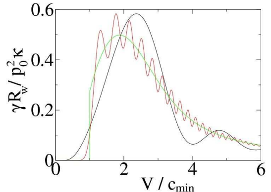
FIG. 1: (Color online) Plot of the wave resistance R_w in units of p_0^2\kappa/\gamma , as a function of the reduced velocity V/c_{\min} = \mathcal{R}\Omega/c_{\min} for different ratios between the trajectory radius \mathcal{R} , and the object size b , as predicted by Eq. (3). The red curve (presenting many oscillations) corresponds to \mathcal{R}/b = 100 , while the black one (with fewer oscillations) corresponds to \mathcal{R}/b = 10 . The green curve displaying a typical discontinuity at V = c_{\min} is the wave drag for a straight uniform motion with velocity V [8]. The object size, b , was set to b = 0.1 \kappa^{-1} .
