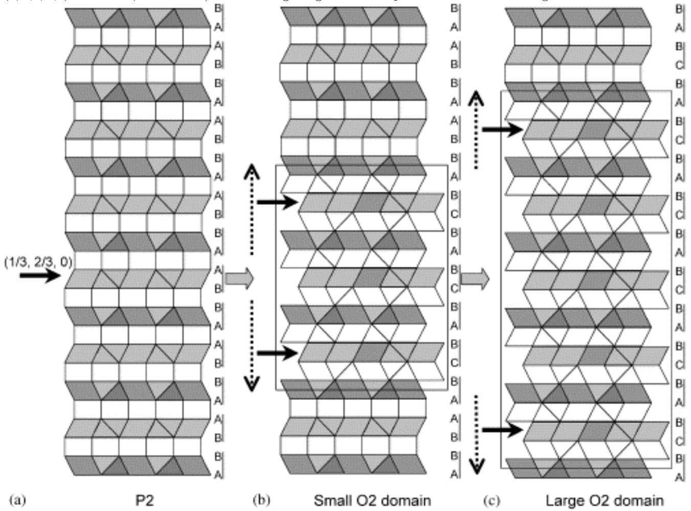
Figure 3: An example of growing of an O2 domain in a P2 crystal, from a BA-type nucleation center in the (1/3, 2/3, 0) direction (black arrow). The same gliding vector is kept for the entire domain growth.
