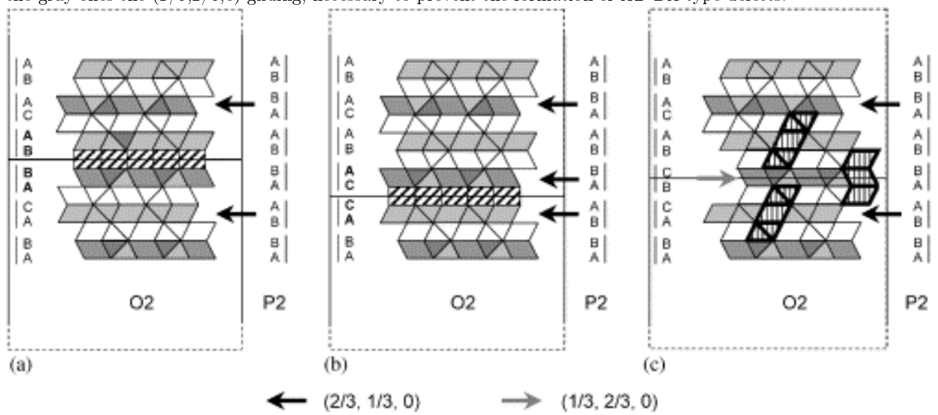
Figure 8: Projection along the (110) direction of the junction between two O2 blocks obtained by the gliding in the same direction of AB -type slabs (for the first) and BA -type slabs (for the second). (a) and (b) show stacking with AB BA -type defects, whereas in (c) these defects are prevented through a slab gliding in the opposite direction. Black arrows represent the (2/3, 1/3, 0) gliding expected for a given growth domain and the gray ones the (1/3, 2/3, 0) gliding, necessary to prevent the formation of AB BA -type defects.
