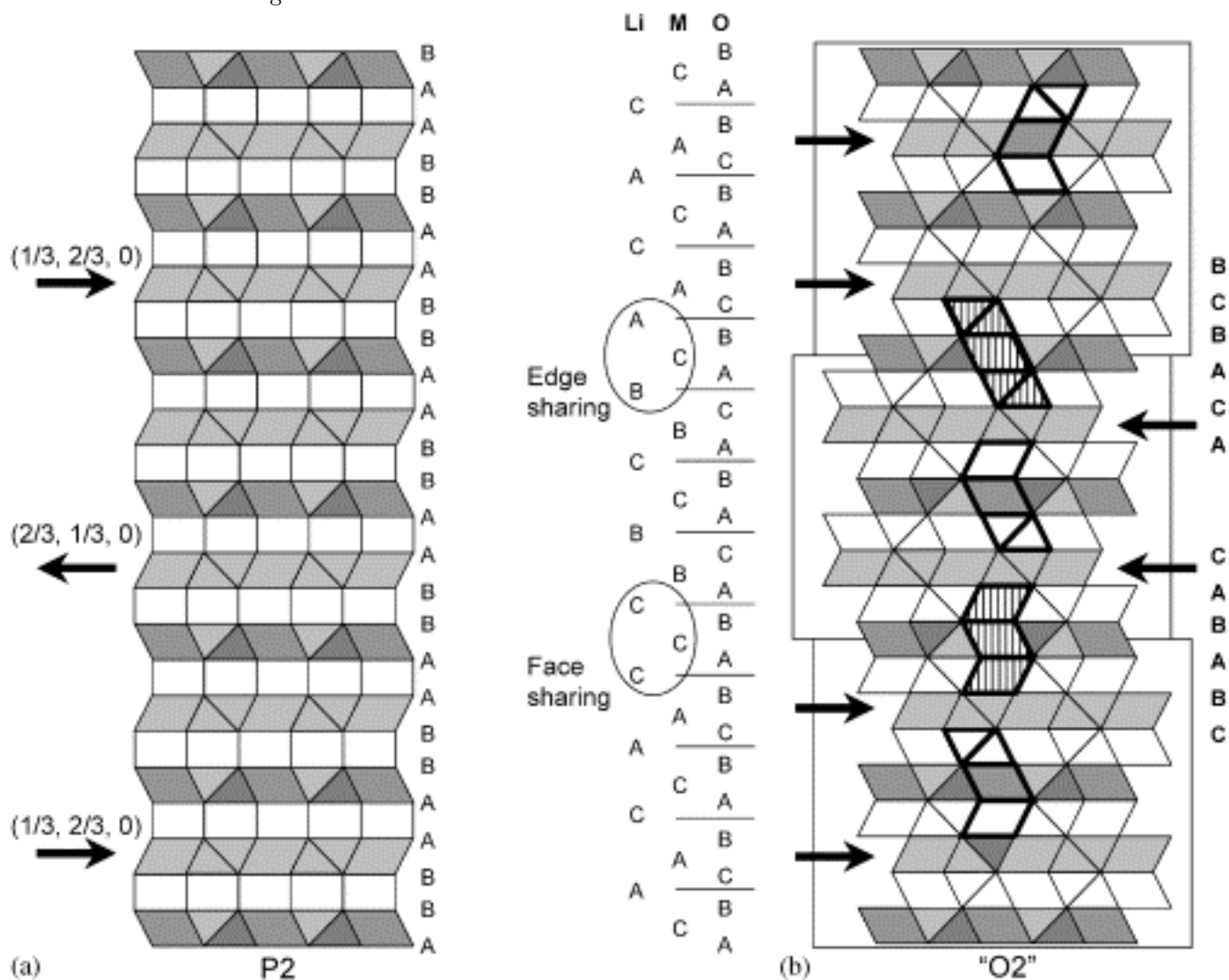
Figure 4: An example of P2→O2 transition section along (110) plane. The lighter slabs are BA-type slabs, whereas the darker slabs are AB-type slabs. The nucleation centers are associated to only one type of slabs (BA for example), the gliding vectors (black arrows) being (1/3, 2/3, 0) or (2/3, 1/3, 0) . The defects appear at the junction between two O2 domains. The classical O2 stacking is highlighted with polyhedra in bold lines and the stacking with defects with hatched polyhedra. Note that, for convenience, the sodium prisms have been drawn with the same height as the lithium octahedra.
