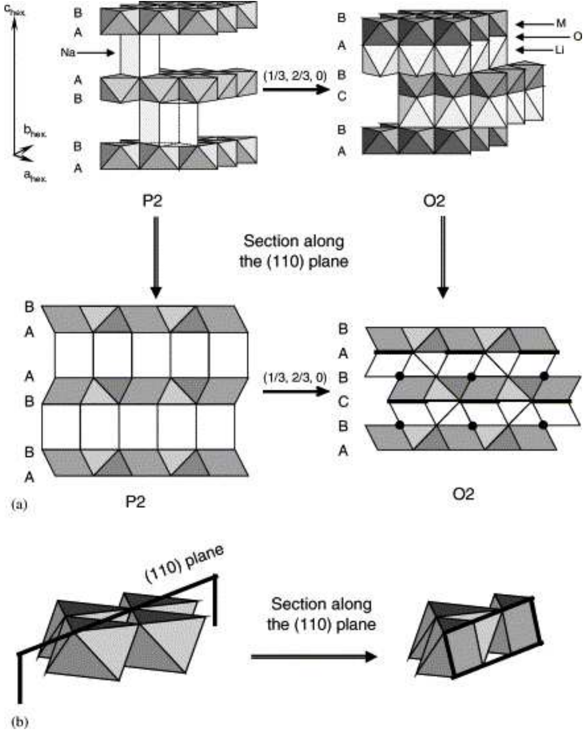
Figure 1: (a) Slab gliding involved in the P2-O2 structural transformation, represented in 3D perspective and in 2D along the (110) direction. A common face appears as a line shared between two parallelograms while a common edge appears as a point in the section. (b) Section along the (110) plane of MO_2 slab.
