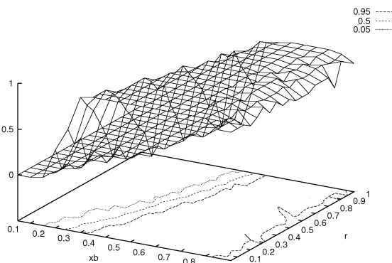
Figure 2: Performances of the SGA on Trap functions.
