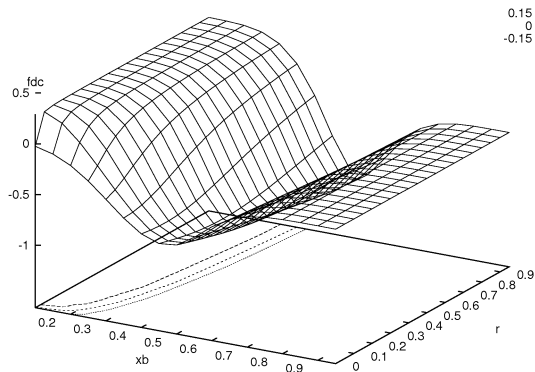
Figure 3: Dual FDC for Trap functions.
