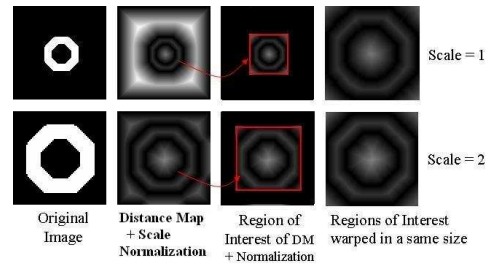
Fig. 6. The new normalization of Distance Map.
