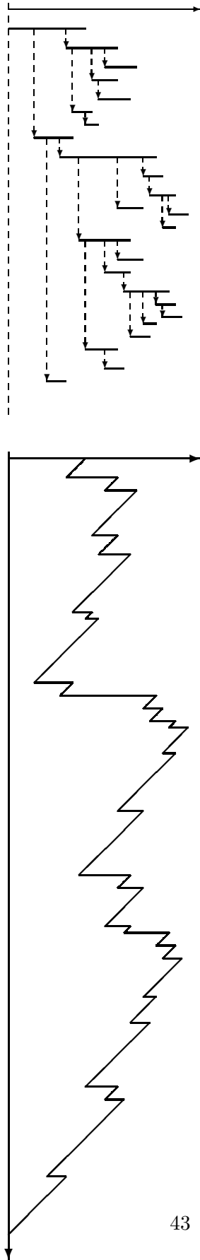
Figure 6: A chronological tree and the associated jumping chronological contour process (JCCP), with jumps in solid line.
