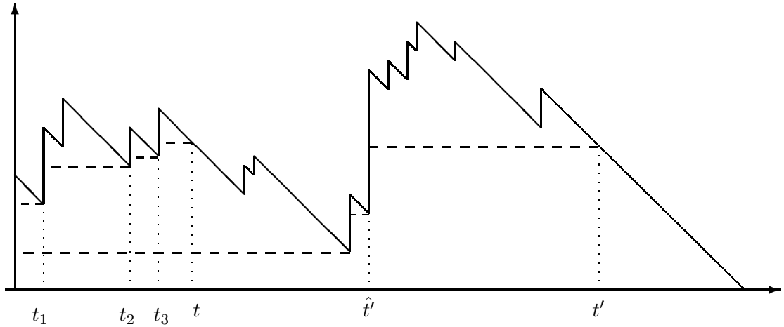
Figure 3: The JCCP of some finite chronological tree with jumps in solid line. Set u = p_1 \circ \varphi^{-1}(t) (resp. v = p_1 \circ \varphi^{-1}(t') ) the individual visited at time t (resp. t' ). The first time when v is visited by the exploration process is \hat{t} . The first visits to the H_t = 3 ancestors of u are also shown.
