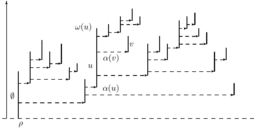
Figure 1: A representation of a chronological tree \mathbb{T} with finite discrete part \mathcal{T} . Horizontal axis has no interpretation, but horizontal arrows indicate filiation; vertical axis indicates chronological levels. Three elements of \mathcal{T} are shown, its root \emptyset , a typical individual v and her mother u . Various elements of \mathbb{T} are shown, its root \rho , the death level \omega(u) of u , as well as the birth levels \alpha(u) and \alpha(v) .
