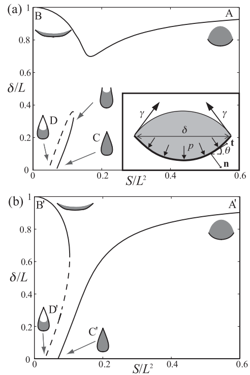
FIG. 4. Distance between the rod tips vs drop volume for different values of the rod length L : (a) L = 3.4L_{EC} reopening of the rod as S decreases; (b) L = 4L_{EC} complete wrapping of the rod around the drop. The inset shows a sketch of a 2D drop deposited on a flexible sheet.
