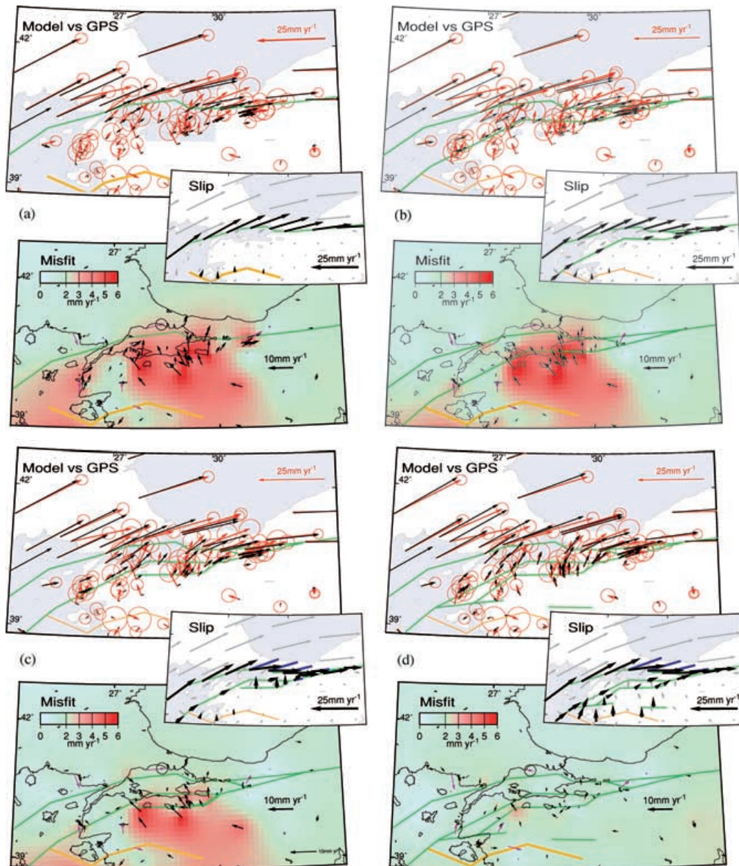
Figure 3. Progressive models of the GPS vectors around the Sea of Marmara. Motion is referenced to fixed Anatolia (as in Fig. 2c). Each figure is composed of three windows. The upper compares the modelled vectors (black) with the observed vectors (red). The ellipses are 80 per cent confidence limits from McClusky et al. (2000). The middle window shows the slip vectors (in black) for different parts of the fault system within the region. In all cases, the models include the larger scale structures shown in Fig. 1(b) and the resultant motions are illustrated with grey arrows. The lower window shows the residual vectors (in black) plus shading (in red) indicating the degree of misfit. The latter is calculated by interpolating between scalar values of the misfit. A few vectors (10 out of 90) are either incoherent with other nearby vectors or have a large error. These are indicated in purple and are not included in the calculation of misfit. The arrowhead of one vector, which is not fitted by the first models, is circled. It might be accounted for by adjusting the locking depth (see text). (a) Only the NNAF is modelled with slip everywhere parallel to and with the amplitude predicted by, the plate motion. Large residuals are visible south of the fault. In the west these are parallel to the plate motion while further east they are orientated perpendicular to it. (b) The SNAF is introduced and the plate motion is redistributed with 80 per cent on the NNAF and 20 per cent on the SNAF. Again the slip is everywhere parallel to the plate motion. The residuals to the south and west of the fault are now reduced, but the misfits to the south of the Sea of Marmara remain. (c) Slip on the NNAF is modified to reduce the component of opening along the eastern part of the Marmara Sea. The overall plate motion direction is shown by blue lines and the new slip direction by black arrows. This leaves a slip deficit with a fault perpendicular component, which is re-distributed along normal faults south of the Sea of Marmara as indicated. This slip partitioning between the two branches of the NAF substantially reduces the residuals. They are now sufficiently small to be within the error ellipses. (d) An optimised model. The condition that no changes can be made to the regional model is now relaxed and some other local faults are added. The strike-slip component on the SNAF is slightly increased and this slip increase extends outside the region of interest to include part of the regional model. Within the region, normal faults with modest opening are added. The locking depth for the NNAF in the northern Sea of Marmara is reduced to 5 km with the result that the vector with the circled head, north of the Marmara, is fitted better. The modifications are discussed in the text and can be justified as consistent with more general tectonic interpretations of the region. However, the residuals are now below the errors quoted for the GPS velocity vectors and thus the interpretation presented in this figure may change as more data is collected.
