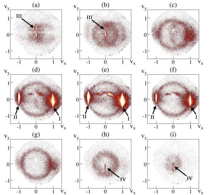
FIG. 2: (Color online) (a-i) Images of the collision of two condensates. Each frame represents a 2.4 ms time slice of the atomic cloud as it passes the plane of the detector ( x - y ). 150 shots have been averaged to obtain these images. The two colliding condensates I, II and the collision sphere are clearly visible. Other features visible in the images are discussed in the text. The axes are marked in units of the recoil velocity.
