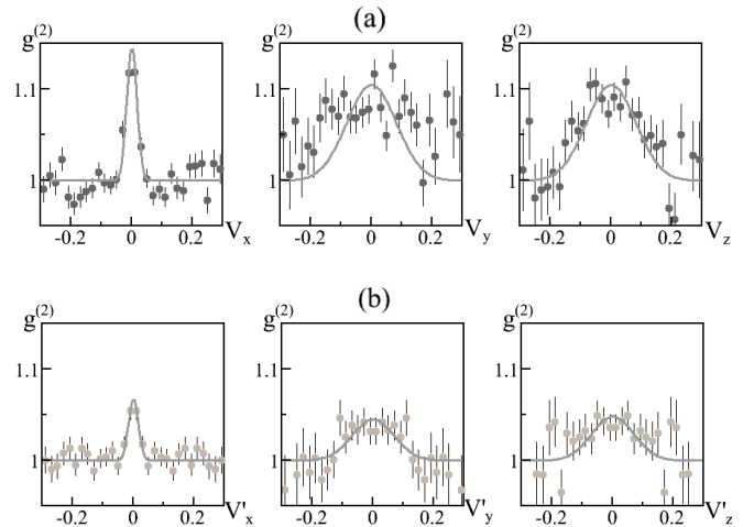
FIG. 3: Back to back (panel a) and collinear (panel b) correlation peaks. (a) Projection of g^{(2)}(\mathbf{V} = \mathbf{V}_1 + \mathbf{V}_2) along the different axes of the experiment and around \mathbf{V} = \mathbf{0} . The projection consists in averaging the correlation in the two other directions over a surface equal to the products of the corresponding correlation lengths. This averaging makes the height smaller than the 3D fitted value \eta^{\text{BB}} = 0.19 \pm 0.02 . The peak is the signature for correlated atoms with opposite velocities. (b) Projection of g^{(2)}(\mathbf{V}' = \mathbf{V}_1 - \mathbf{V}_2) along the different axes of the experiment. This peak is due to the Hanbury Brown and Twiss bunching effect. All velocities are expressed in units of the recoil velocity.
