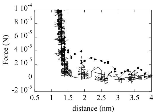
FIG. 3: Normal load as a function of hexadecane thickness for two approach velocities: 0.2 \text{ nm}\cdot\text{s}^{-1} (solid line) and 5 \text{ nm}\cdot\text{s}^{-1} (dashed line with symbols).
