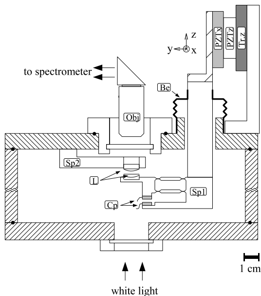
FIG. 1: Mechanical arrangement of the surface force apparatus. Two crossed cylindrical lenses (L) are mounted in springs (Sp1 and Sp2), the deflexion of which is measured by means of capacitive displacement sensors (Cp). The normal load spring (Sp1) is attached to a shaft that can be moved horizontally by means of a long travel piezoactuator (PZTx), and vertically via a two stage mechanism composed of a piezoactuator (PZTz) and a motorized translation stage (Tr.z). A rubber bellow (Be) is used to ensure air-tightness of the vessel while allowing for normal and tangential displacement of the shaft.
