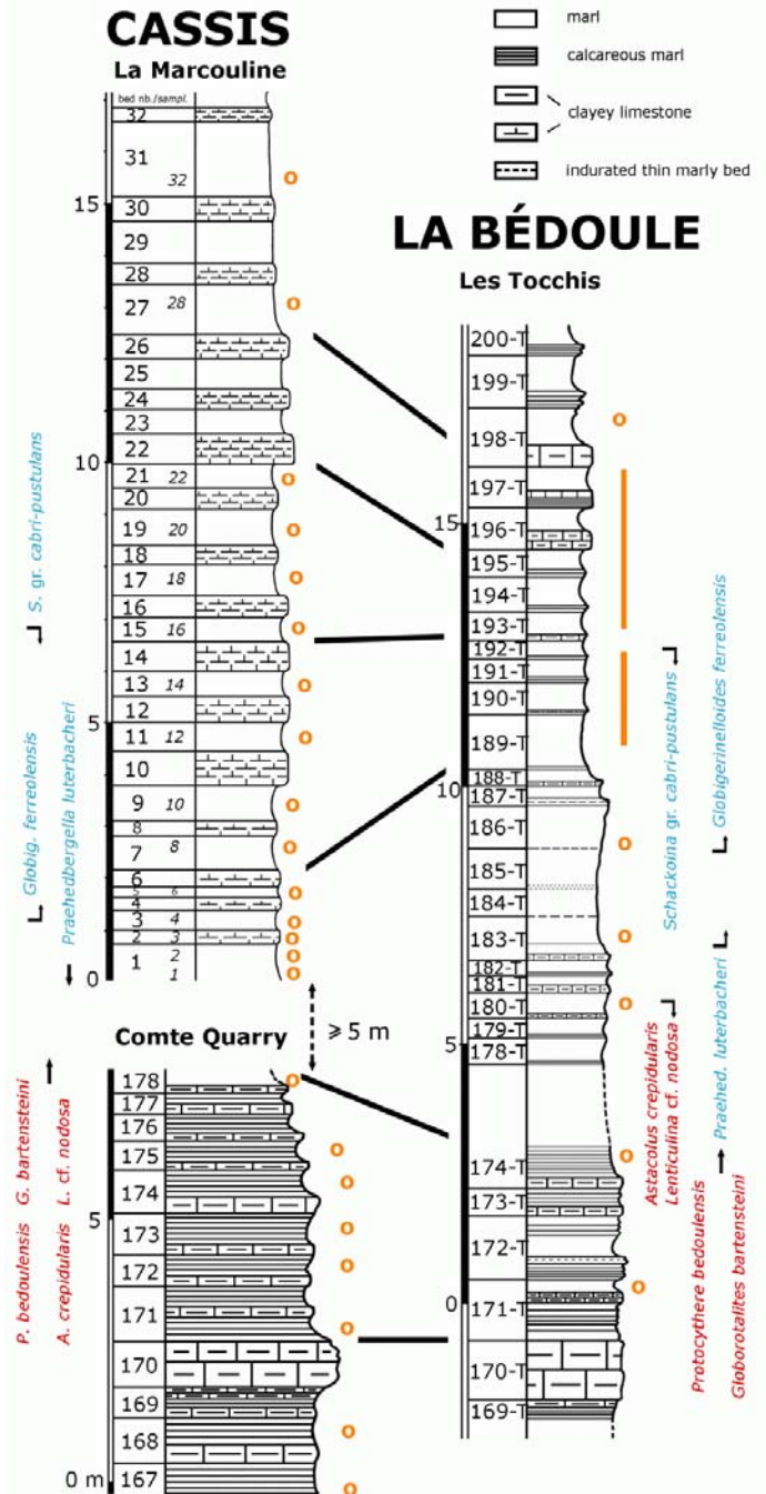
Figure 5: Correlation of the three sections (Comte, Tocchis, Marcoulaine) that permits a reconstitution of the sequence from uppermost Bedoulian to lowermost Gargasian. The boundary between the two substages is fixed at bed 178 (cf. CONTE, 1994).
