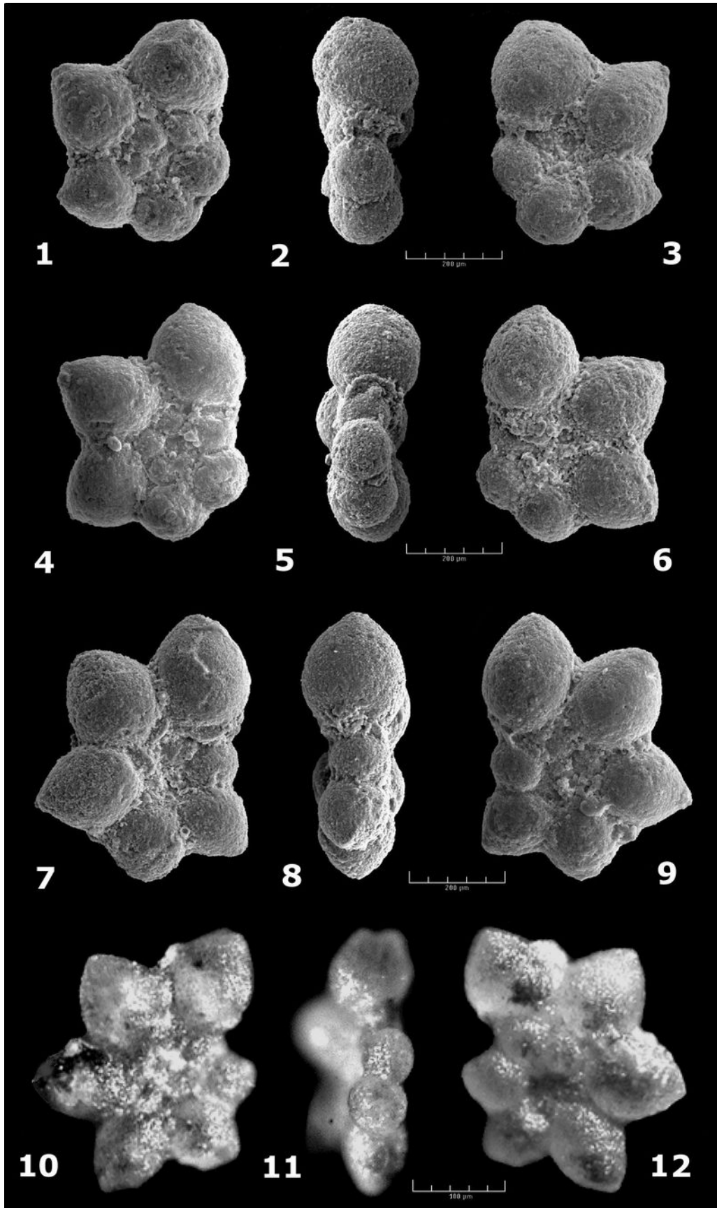
1-9. " Globigerinelloides " gr. bizonae (CHEVALIER) – saunderi (BOLLI). 3 specimens showing various modes of coiling (from trochospiral to subplanispiral). Lowermost Gargasian, Luterbacheri Zone, Les Tocchis section (La Bédoule), bed 189-T.
