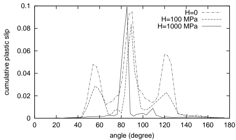
Figure 3: Amount of equivalent plastic slip along a half circle close to the crack tip for three different values of the Cosserat extra-hardening parameter H .
