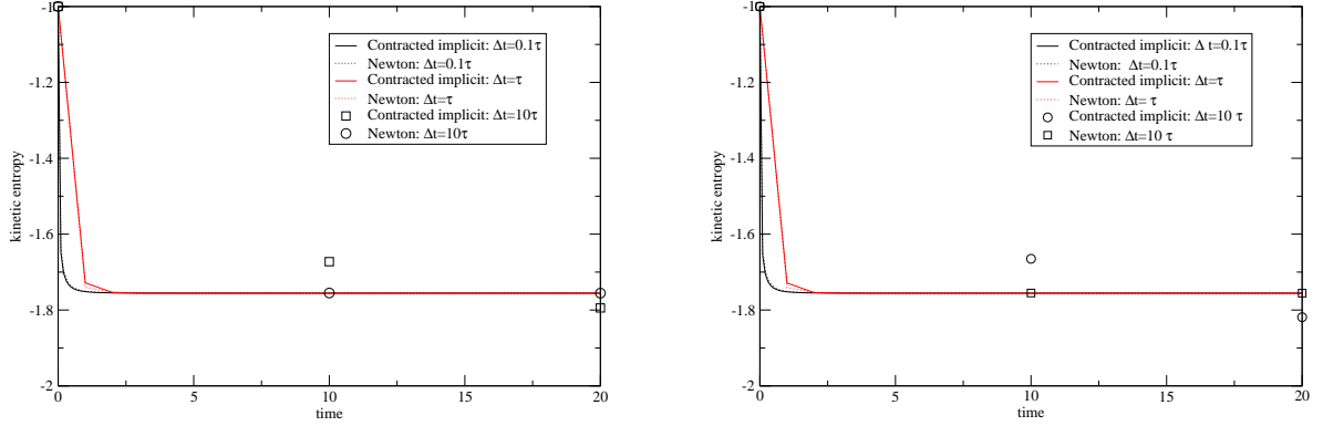
Figure 5: Test 2. Kinetic entropy for contracted implicit scheme and Newton method, \mathcal{S}_1 vs \mathcal{S}_3
