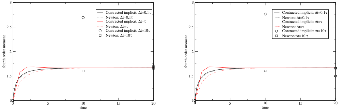
Figure 6: Test 2. Fourth order moment for contracted implicit scheme and Newton method, \mathcal{S}_1 vs \mathcal{S}_3
