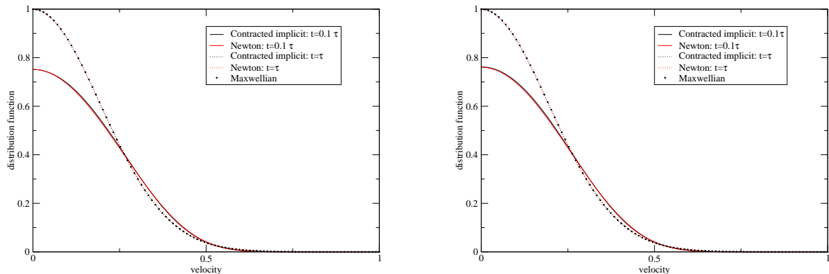
Figure 3: Test 1. Distribution function, \Delta t = \tau , \mathcal{S}_1 vs \mathcal{S}_3
