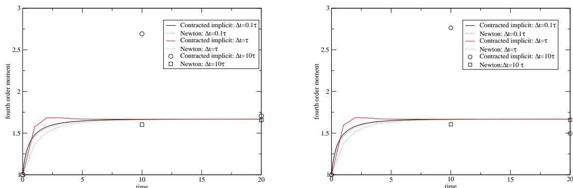
Figure 6: Test 2. Fourth order moment for contracted implicit scheme and Newton method, \mathcal{S}_1 vs \mathcal{S}_3
