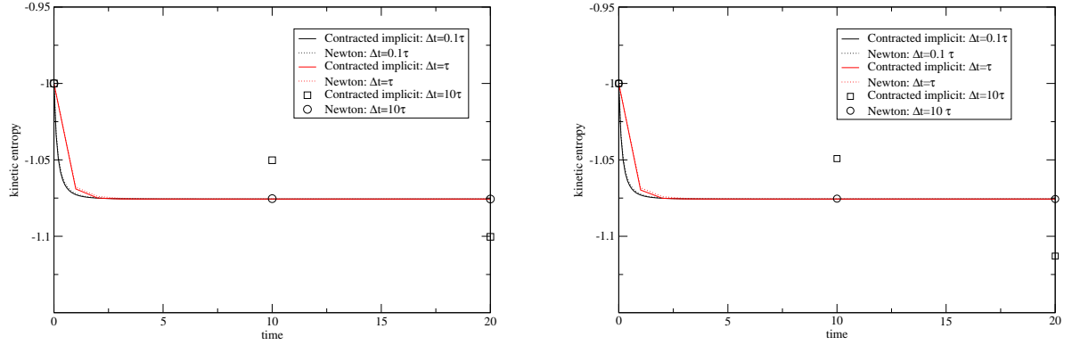
Figure 1: Test 1. Kinetic entropy for contracted implicit scheme and Newton method, \mathcal{S}_1 vs \mathcal{S}_3
