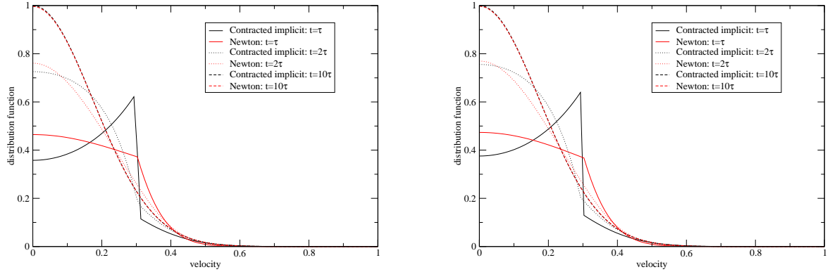
Figure 4: Test 2. Distribution function, \Delta t = \tau , \mathcal{S}_1 vs \mathcal{S}_3
