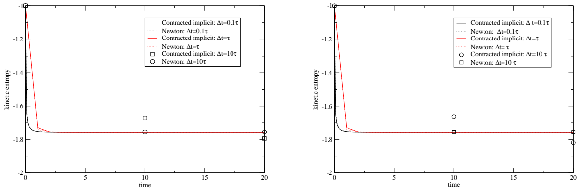
Figure 5: Test 2. Kinetic entropy for contracted implicit scheme and Newton method, \mathcal{S}_1 vs \mathcal{S}_3
