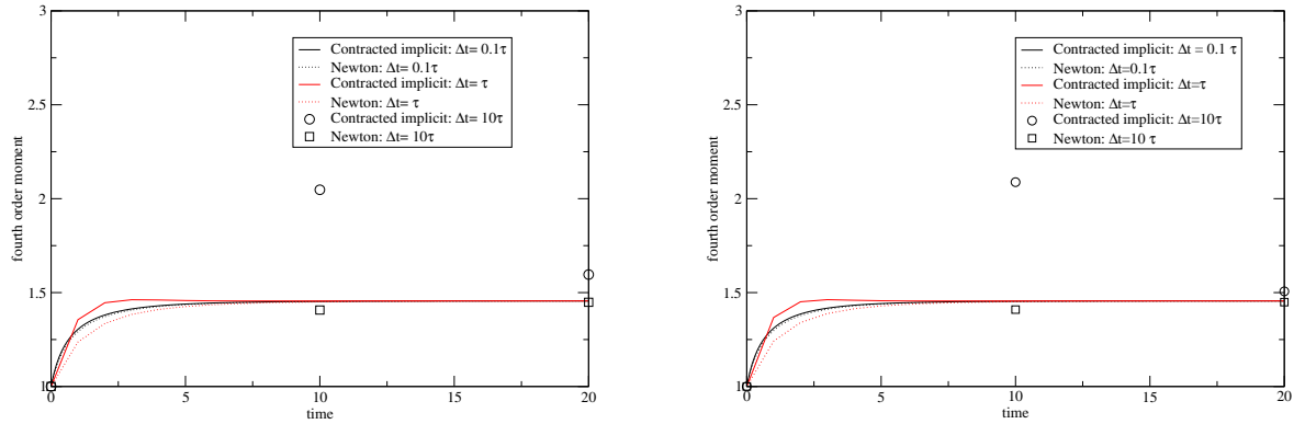
Figure 2: Test 1. Fourth order moment for contracted implicit scheme and Newton method, \mathcal{S}_1 vs \mathcal{S}_3
