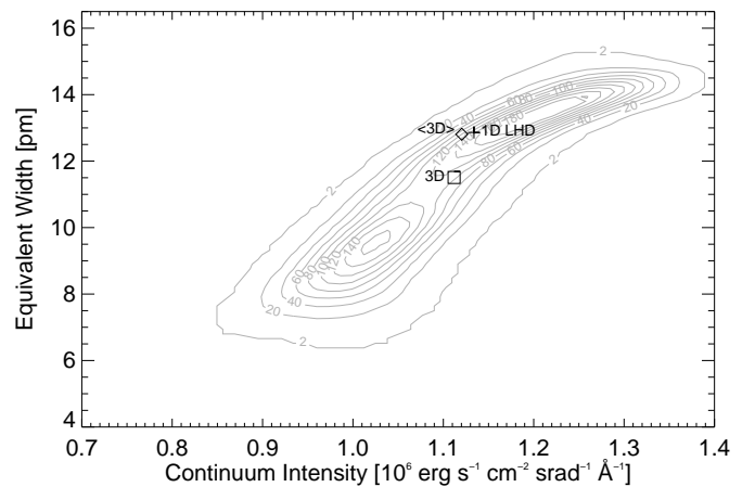
Fig. 4. Sun: same as Fig. 3 for the solar case. The micro-turbulent velocity for the 1D models is 1.0 \text{ km s}^{-1} .
