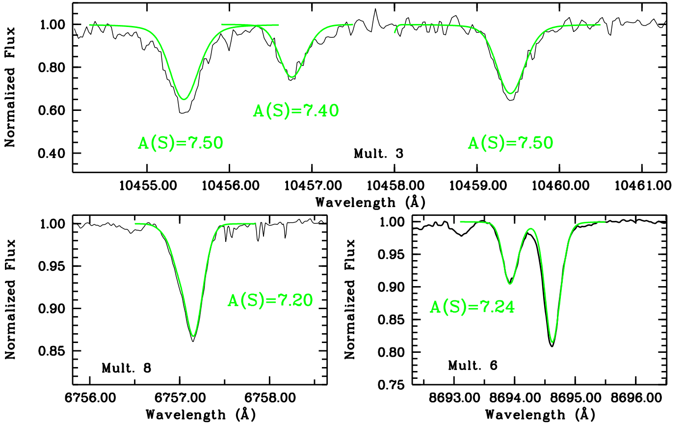
Fig. 5. Procyon: synthetic spectra (green thick line) based on the 3D model are over-imposed on the observed (black solid line) ones.
