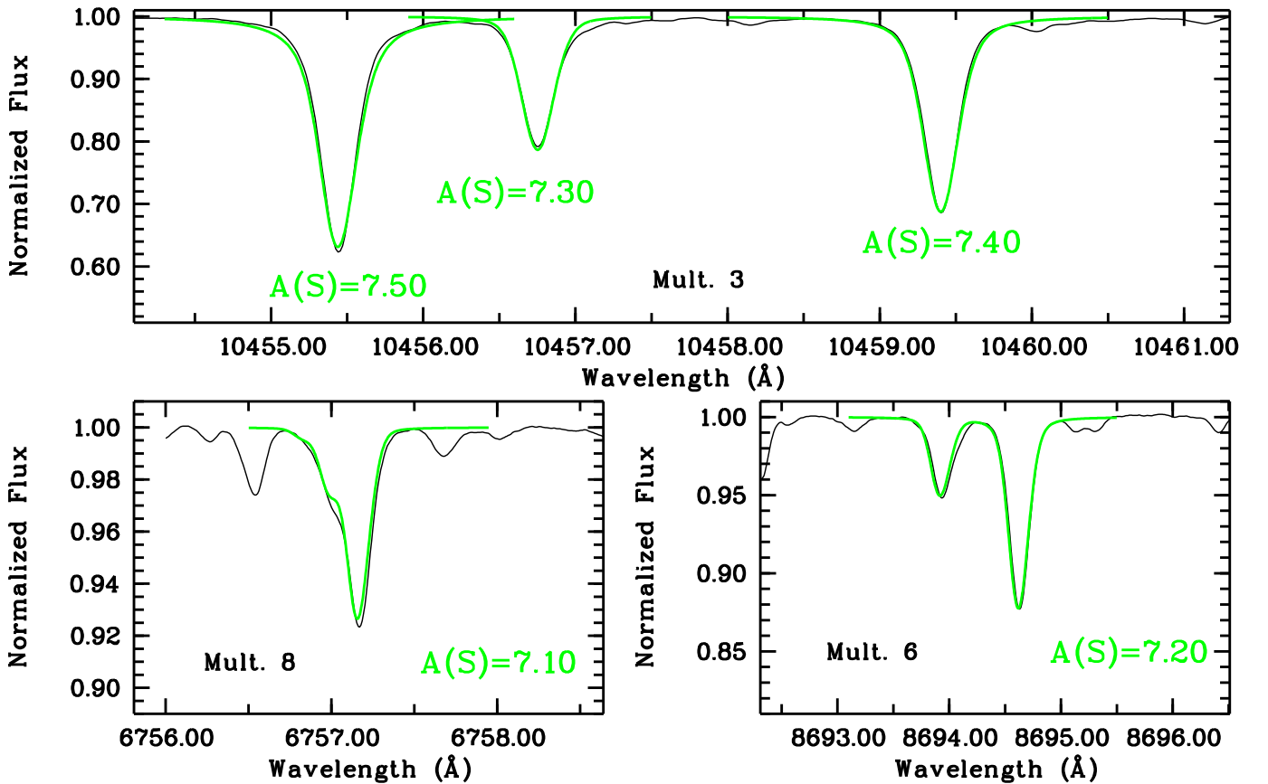
Fig. 1. Sun: synthetic spectra (green/grey thick solid line) based on the 3D model atmosphere are over-imposed on the observed (black solid line) solar flux spectrum of Kurucz.
