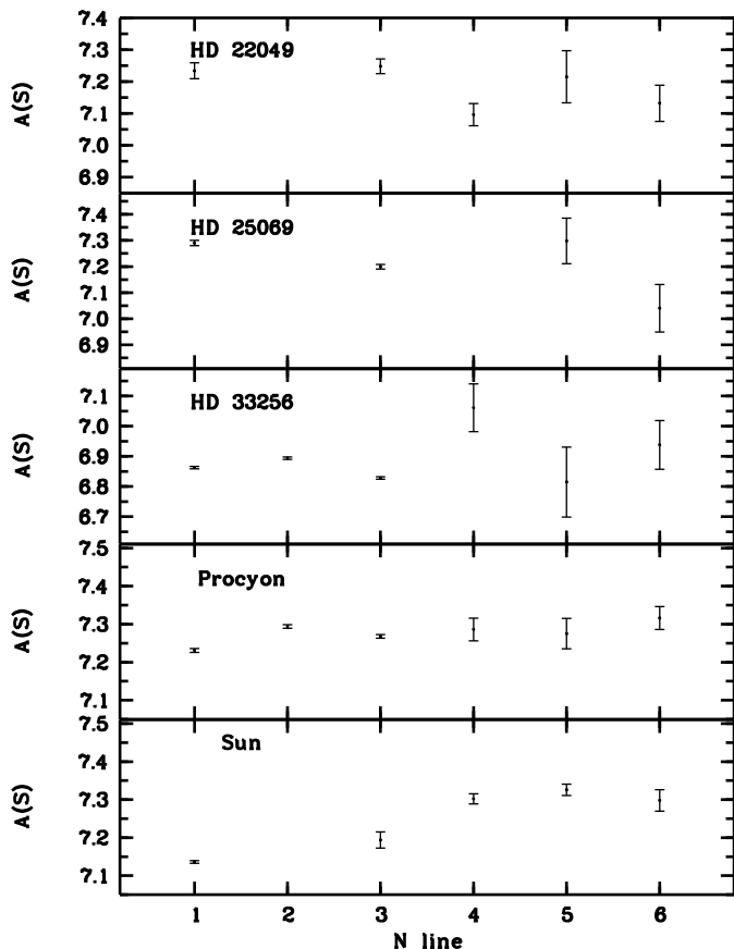
Fig. 6. For each star, A(S) is plotted as a function of the number of the line: 1 is the 675.7 nm triplet, 2 the 869.3 nm line, 3 the 869.4 nm line, 4 the 1045.5 nm line, 5 the 1045.6 nm line and 6 the 1045.9 nm line. For the Sun the error bar is related to the statistical error coming from the two observed flux spectra. For the other stars it is related to the S/N through Eq. (1).
