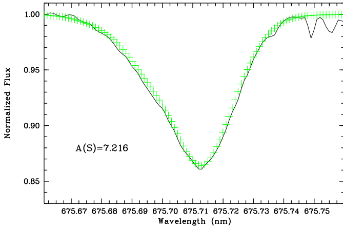
Fig. 2. Procyon: the 3D fit (green/grey crosses) is over-imposed on the observed spectrum (black solid line) for the S I 675.7 nm triplet.
