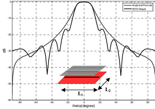
Fig. 3. Radiation pattern of a infinitely long current source inside the cavity with D_1=D_2=24\text{mm} ; L_2=1\text{m} ; surface of metallic wires with a/Pt=5\% ; Pt=12\text{mm} , a : diameter of wires, Pt : distance between wires
