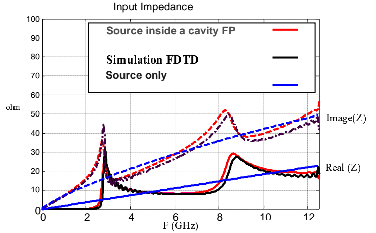
Fig.7. Input impedance of a infinitely long current source placed inside a cavity
