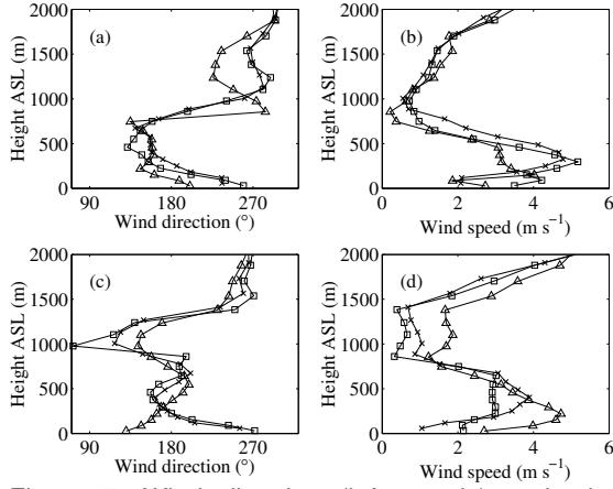
Figure 7: Wind direction (left panels) and wind speed (right panels) at the three locations indicated on Fig.2 as derived from the model outputs at 1100 (panels a and b) and 1600~UTC (panels c and d).
