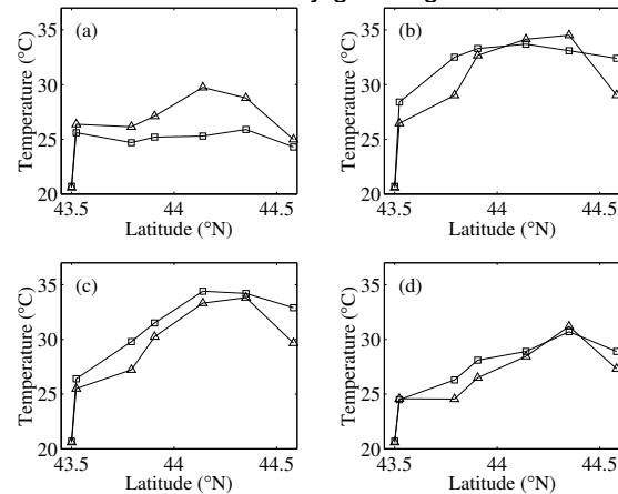
Figure 3: Horizontal cross section of the observed (squares) and simulated (triangles) surface temperature along the line IST, STR, AVI, ORA, STP, MON (see Fig.2) on J25 at 0800 (panel a), 1100 (panel b), 1300 (panel c) and 1600 UTC (panel d). The observed temperature is derived from the meteorological surface station network of Météo-France.
