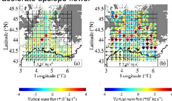
Figure 10: Horizontal and vertical mass fluxes calculated from Mésos-NH at 1400 UTC. Arrows are fit within the importance of the horizontal mass flux and indicate its direction. Color represents the sign and the importance of the vertical mass flux.
