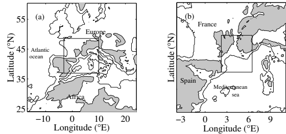
Figure 1: (a) Map of the coarsest domain of the simulation with its nested smaller domain (domain 2) in the rectangle. The topography is shaded in grey when higher than 500 m. (b) Domain 2 with its nested smaller domain (domain 3) in the rectangle.
