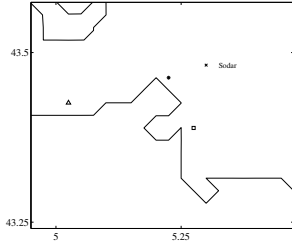
Figure 8: zoom of the topography near Marseille. The thick cross indicates the location of the sodar at Vallon d'Ol. The triangle, star and square indicate the locations where vertical profiles of the wind are extracted from the simulation.
