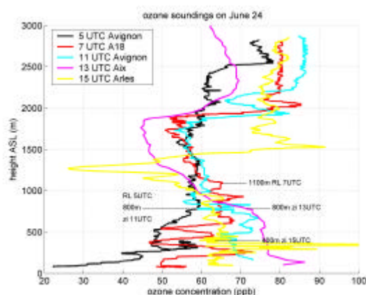
Fig. 5: Ozone profiles from various soundings during June 24 over the ESCOMPTE area. RL means residual layer.
