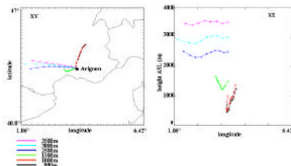
Fig. 6 : back trajectories at various level in horizontal view (left) and vertical view (right) for June 24. The particle arrived in Avignon and points correspond to every hour position.
